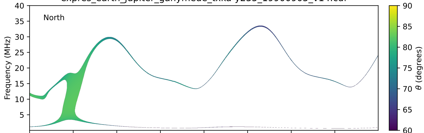
expres_earth_jupiter_ganymede_txka-y235_19900905_v14.cdf
