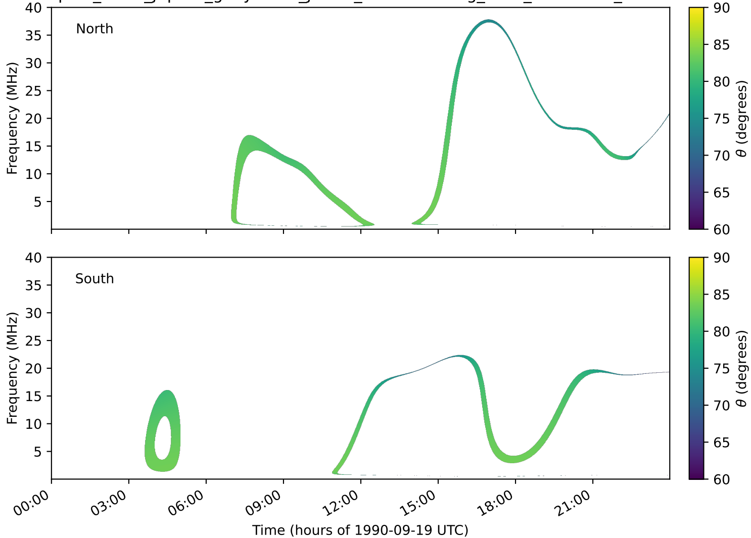
expres_earth_jupiter_ganymede_jrm33_lossc-wid1deg_3kev_19900919_v11.cdf
