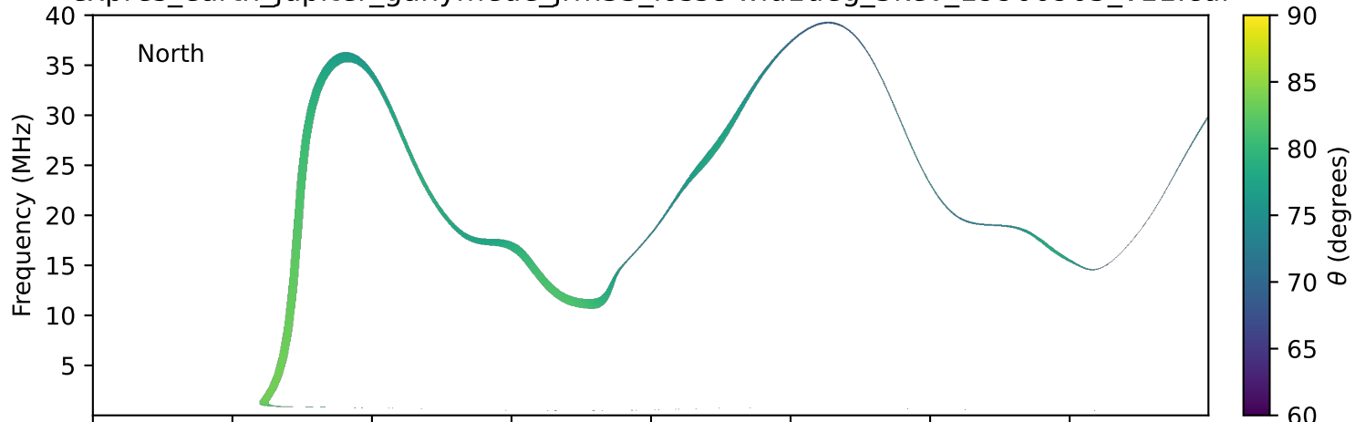
expres_earth_jupiter_ganymede_jrm33_lossc-wid1deg_3kev_19900905_v11.cdf
