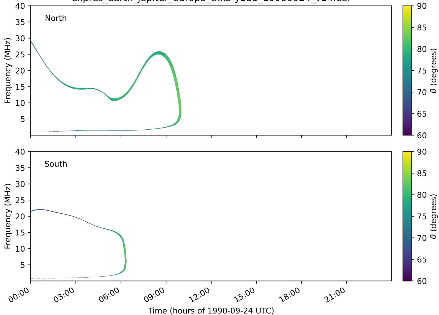
expres_earth_jupiter_europa_txka-y235_19900924_v14.cdf
