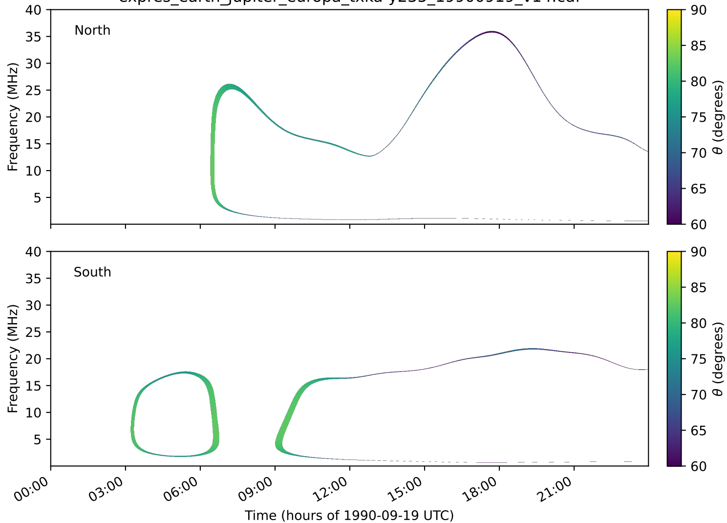
expres_earth_jupiter_europa_txka-y235_19900919_v14.cdf
