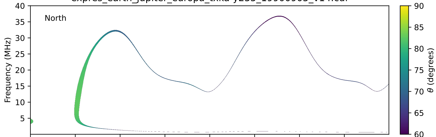
expres_earth_jupiter_europa_txka-y235_19900905_v14.cdf
