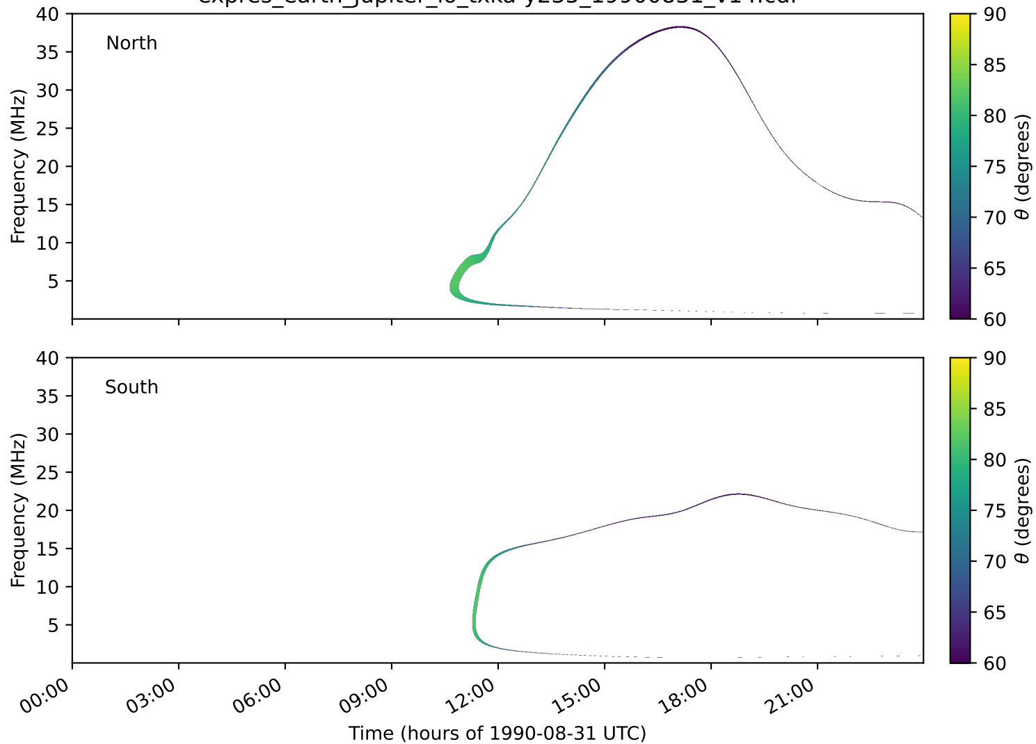
expres_earth_jupiter_io_txka-y235_19900831_v14.cdf
