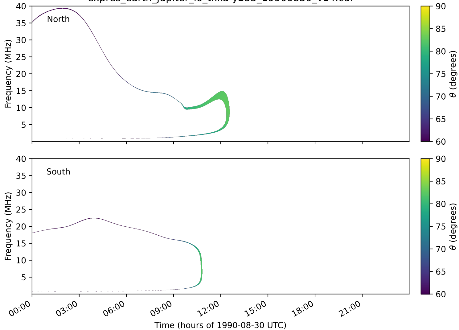
expres_earth_jupiter_io_txka-y235_19900830_v14.cdf
