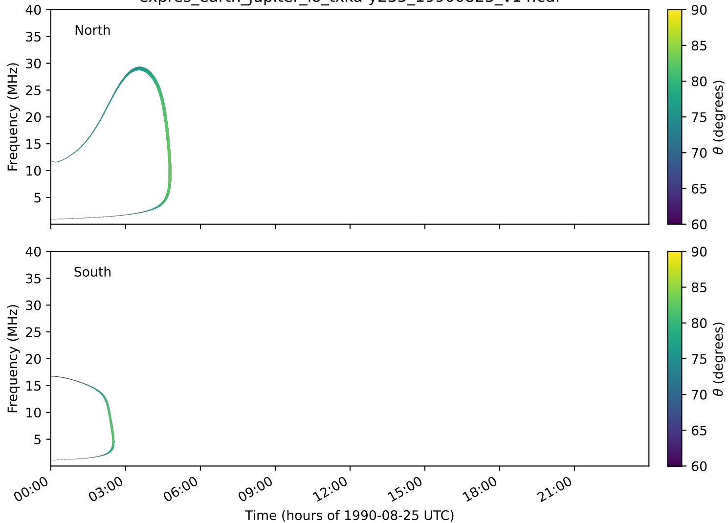
expres_earth_jupiter_io_txka-y235_19900825_v14.cdf
