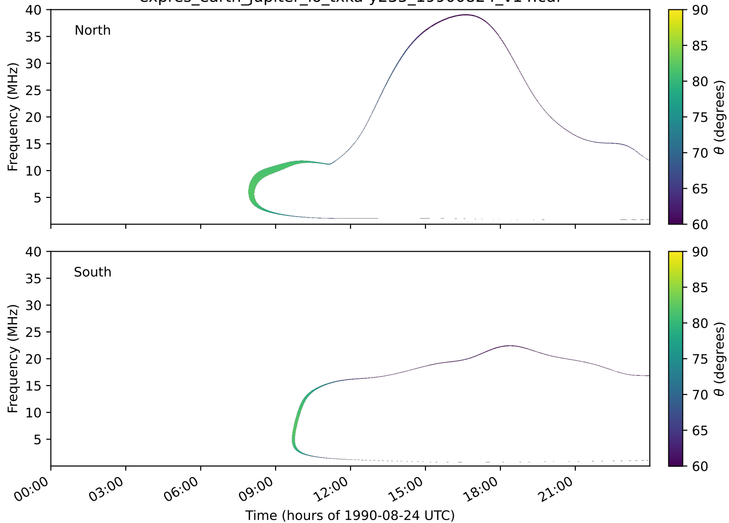
expres_earth_jupiter_io_txka-y235_19900824_v14.cdf
