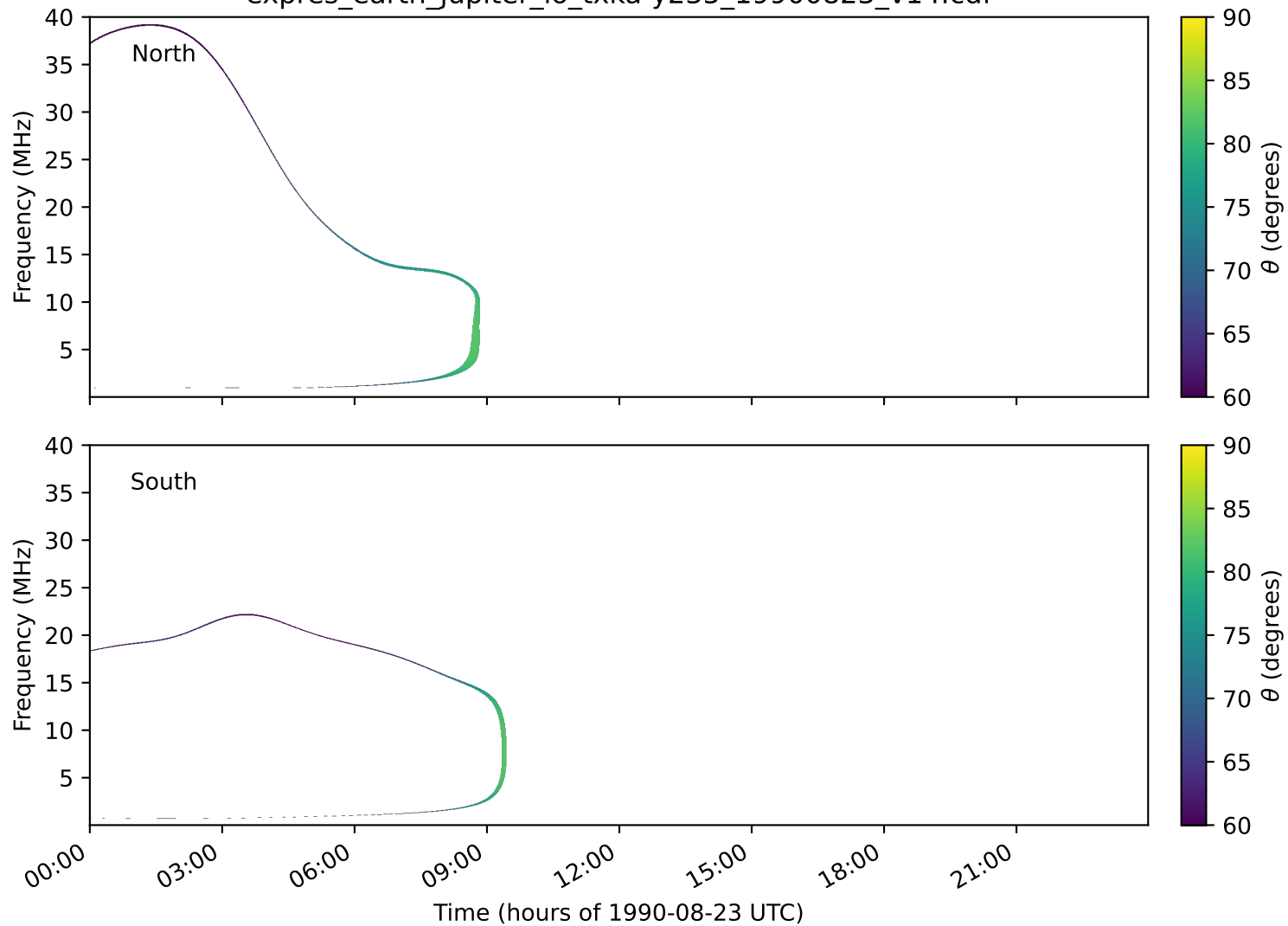
expres_earth_jupiter_io_txka-y235_19900823_v14.cdf
