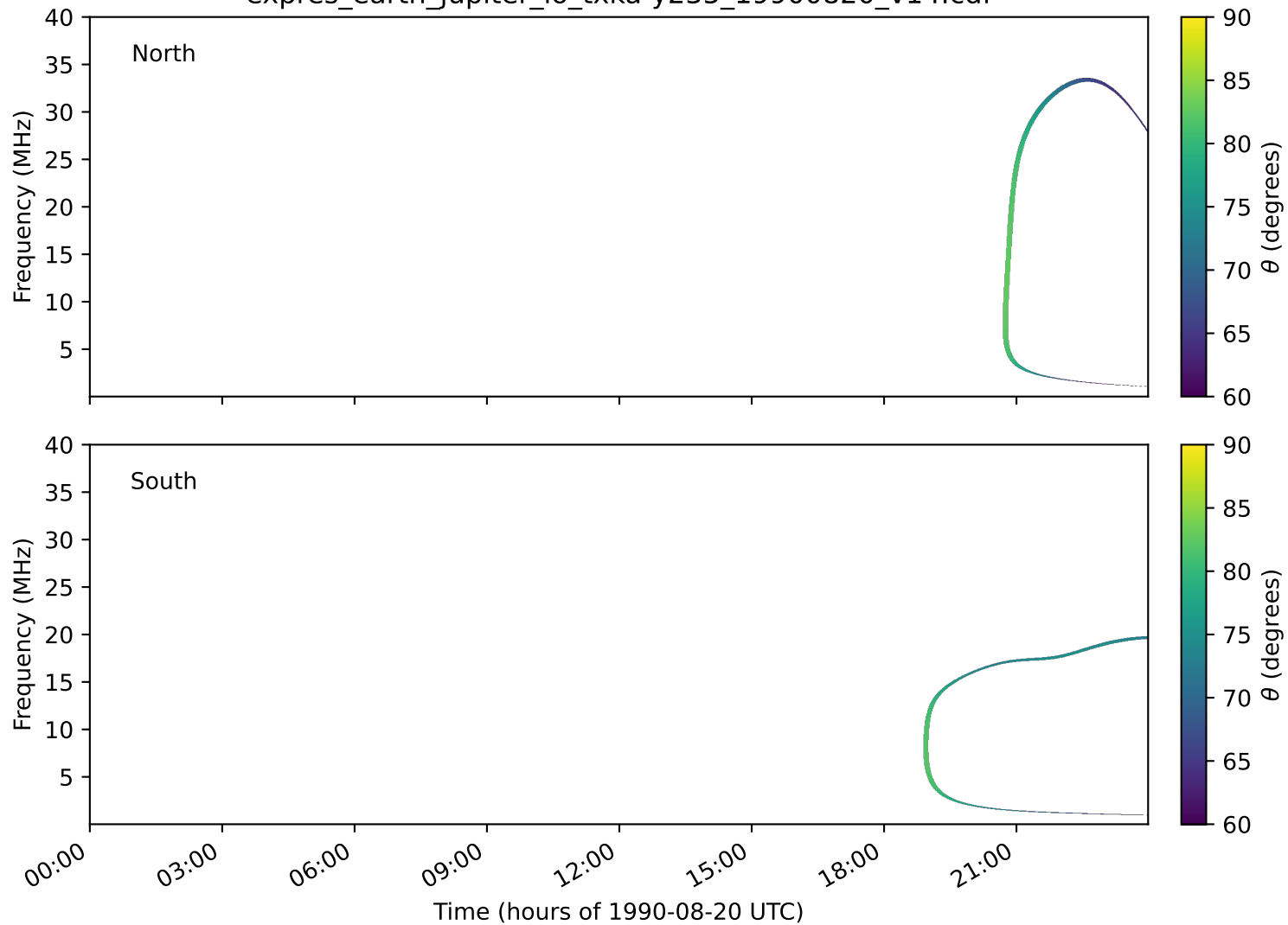
expres_earth_jupiter_io_txka-y235_19900820_v14.cdf
