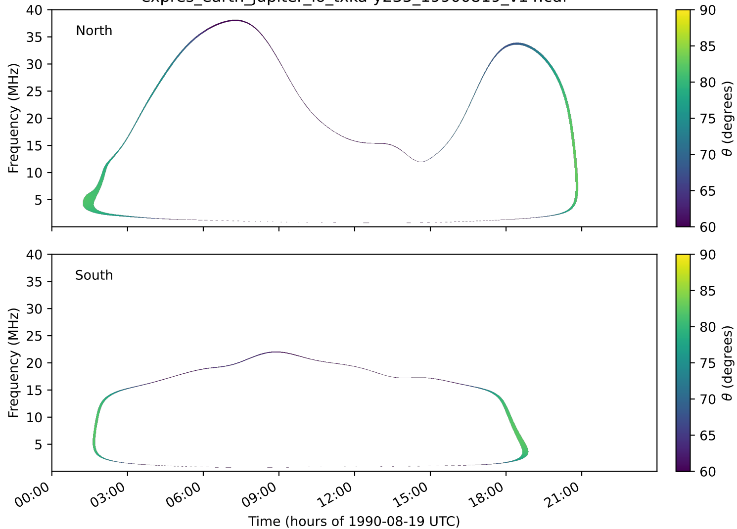
expres_earth_jupiter_io_txka-y235_19900819_v14.cdf
