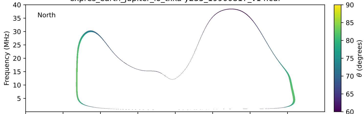
expres_earth_jupiter_io_txka-y235_19900817_v14.cdf
