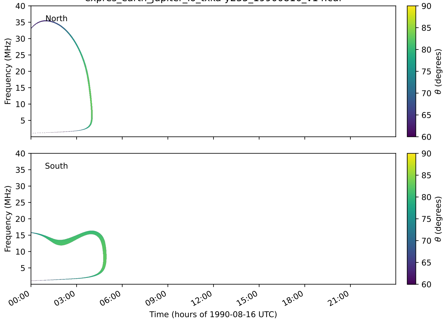
expres_earth_jupiter_io_txka-y235_19900816_v14.cdf
