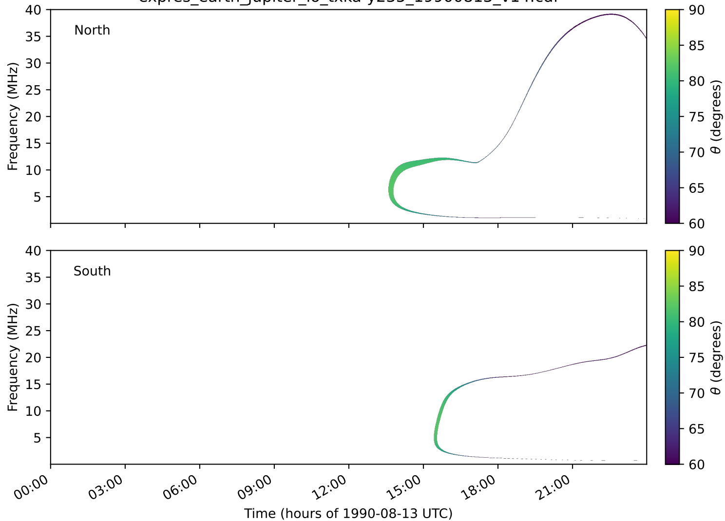
expres_earth_jupiter_io_txka-y235_19900813_v14.cdf
