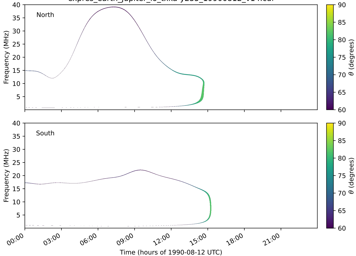
expres_earth_jupiter_io_txka-y235_19900812_v14.cdf
