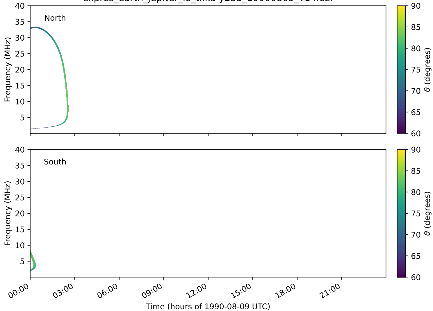
expres_earth_jupiter_io_txka-y235_19900809_v14.cdf
