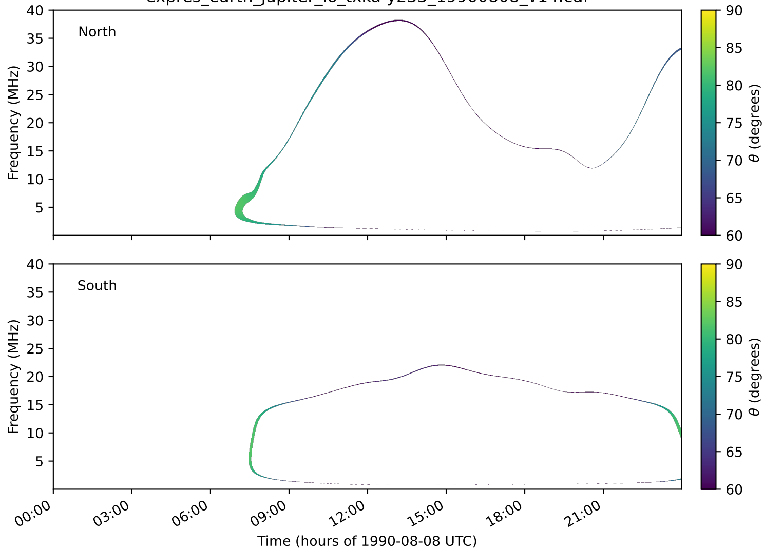
expres_earth_jupiter_io_txka-y235_19900808_v14.cdf
