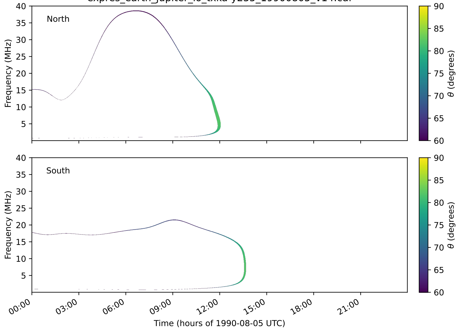
expres_earth_jupiter_io_txka-y235_19900805_v14.cdf
