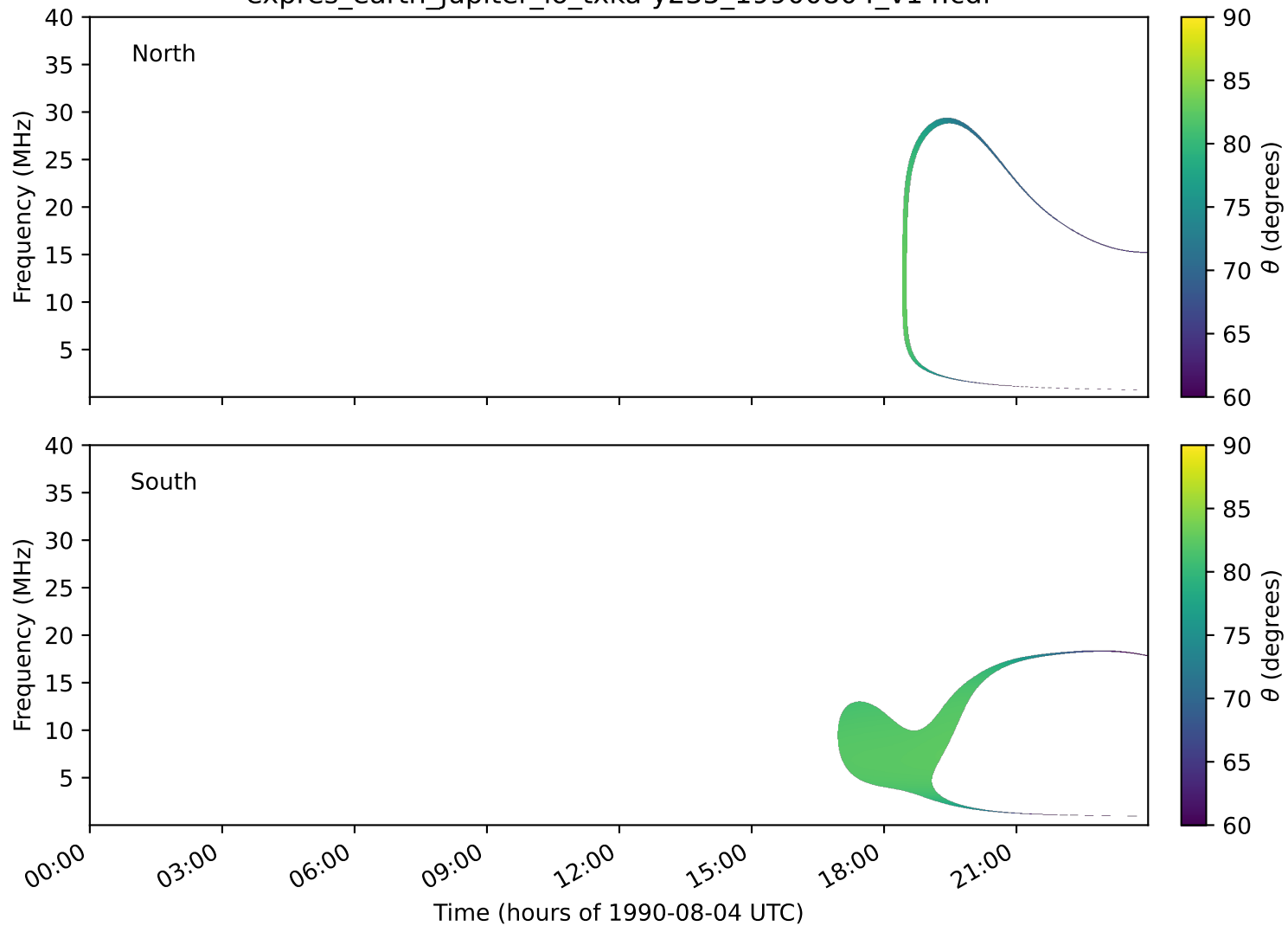
expres_earth_jupiter_io_txka-y235_19900804_v14.cdf
