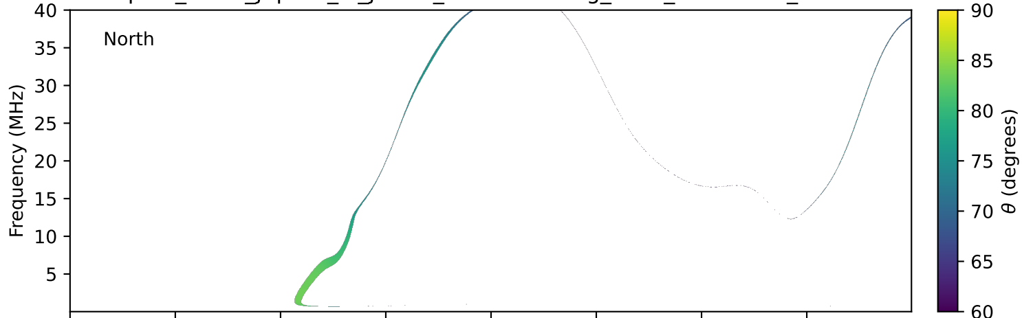
expres_earth_jupiter_io_jrm33_lossc-wid1deg_3kev_19900808_v11.cdf
