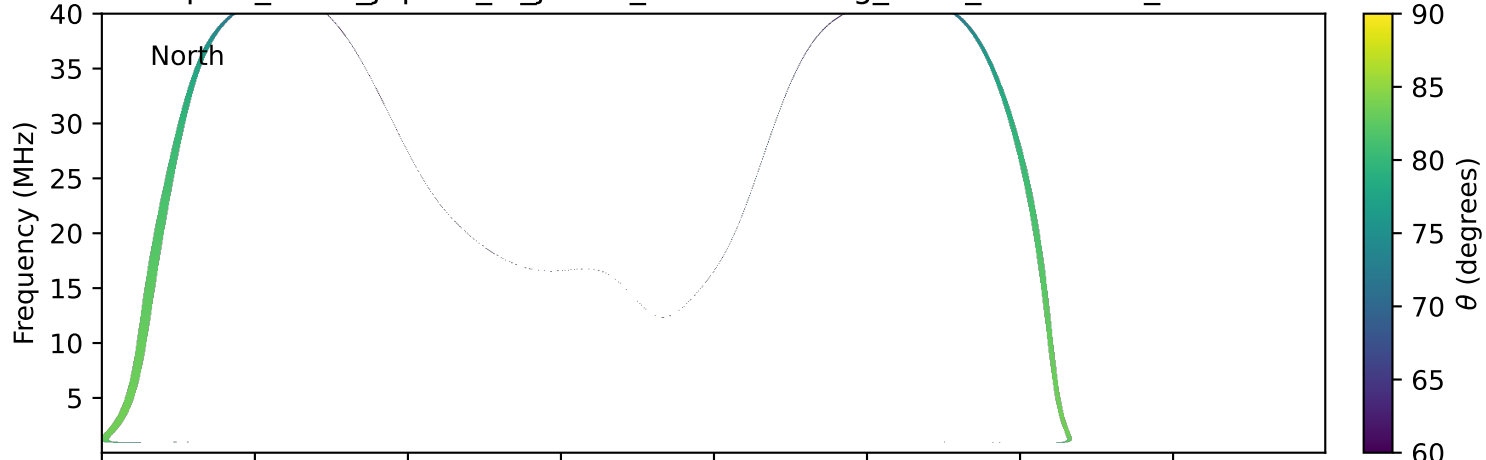
expres_earth_jupiter_io_jrm33_lossc-wid1deg_3kev_19900803_v11.cdf
