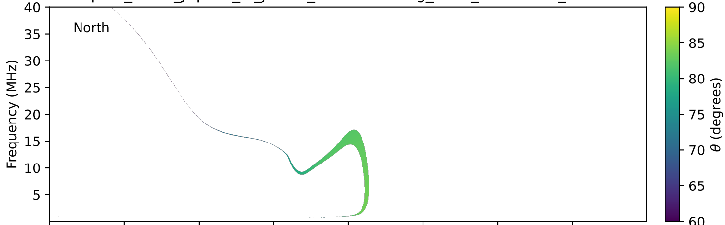
expres_earth_jupiter_io_jrm09_lossc-wid1deg_3kev_19900830_v11.cdf
