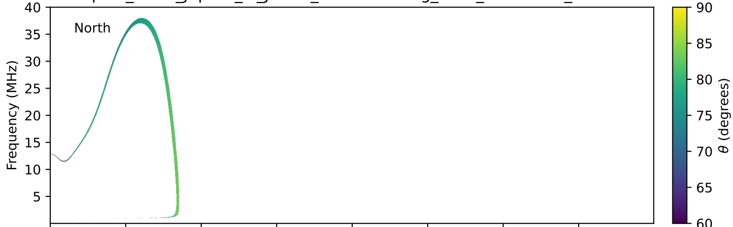
expres_earth_jupiter_io_jrm09_lossc-wid1deg_3kev_19900825_v11.cdf
