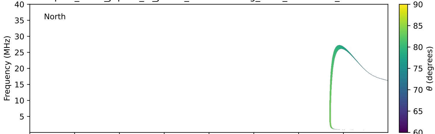
expres_earth_jupiter_io_jrm09_lossc-wid1deg_3kev_19900811_v11.cdf
