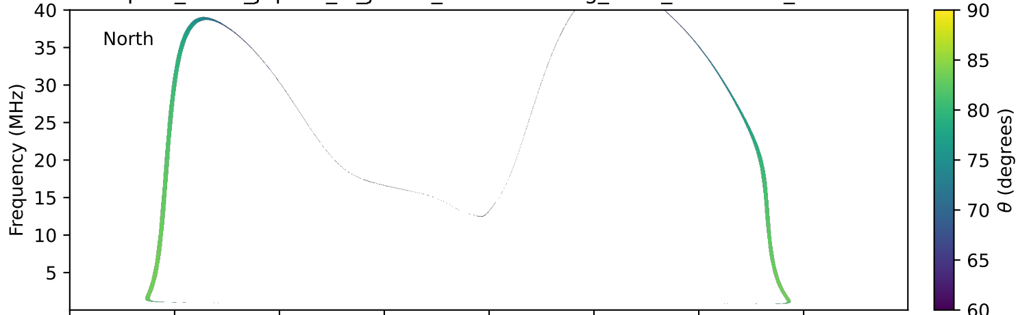
expres_earth_jupiter_io_jrm09_lossc-wid1deg_3kev_19900810_v11.cdf
