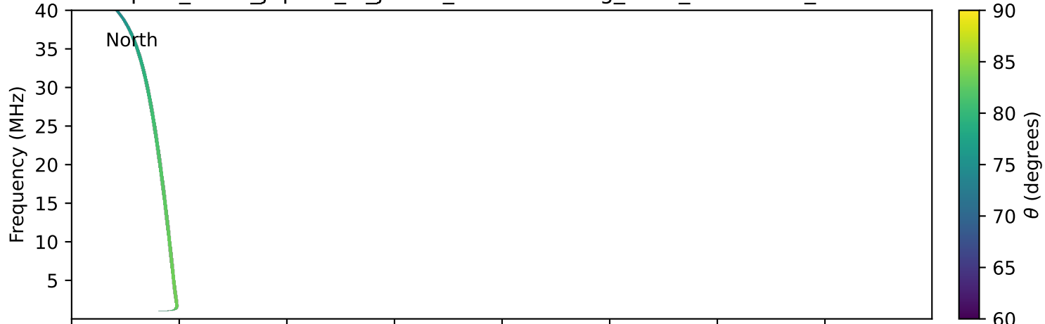
expres_earth_jupiter_io_jrm09_lossc-wid1deg_3kev_19900809_v11.cdf
