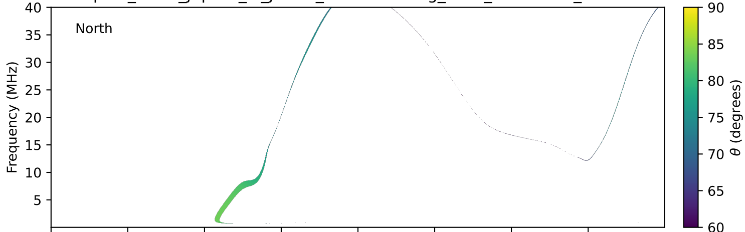
expres_earth_jupiter_io_jrm09_lossc-wid1deg_3kev_19900808_v11.cdf
