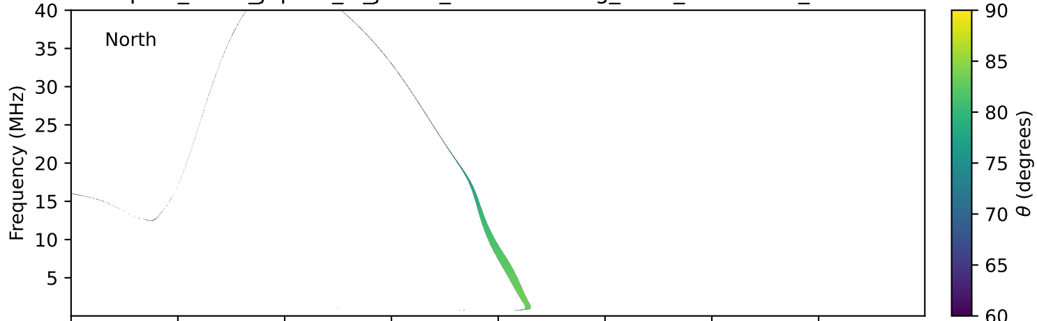
expres_earth_jupiter_io_jrm09_lossc-wid1deg_3kev_19900805_v11.cdf
