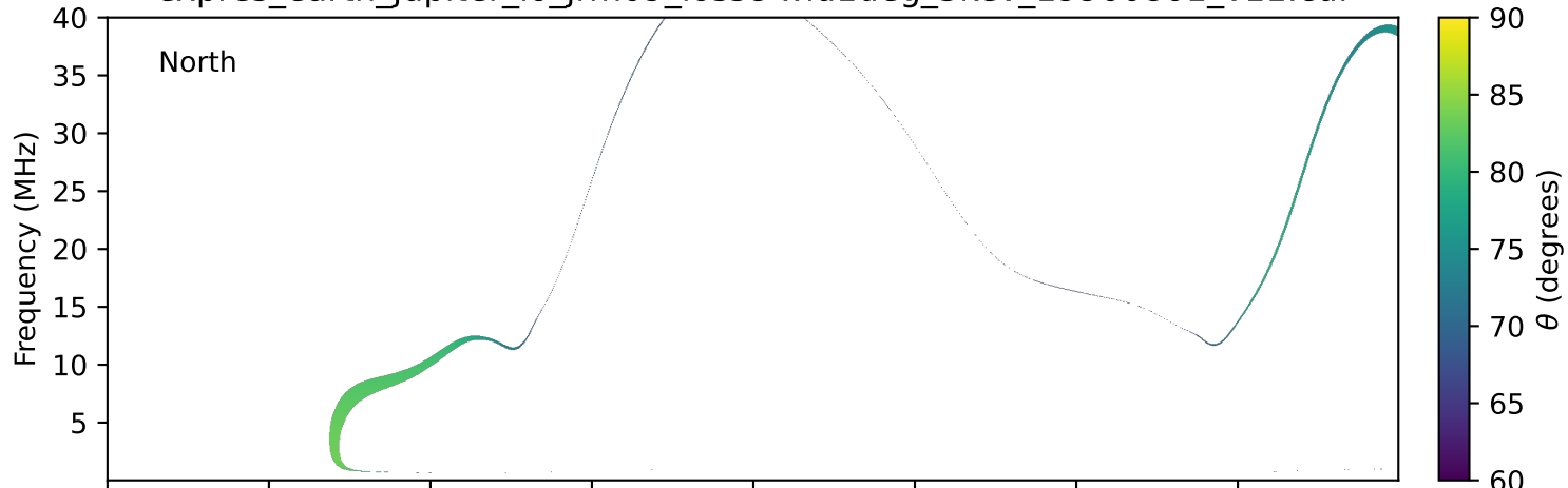
expres_earth_jupiter_io_jrm09_lossc-wid1deg_3kev_19900801_v11.cdf
