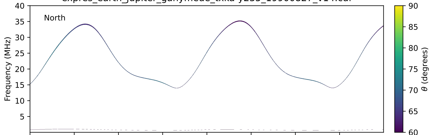
expres_earth_jupiter_ganymede_txka-y235_19900827_v14.cdf
