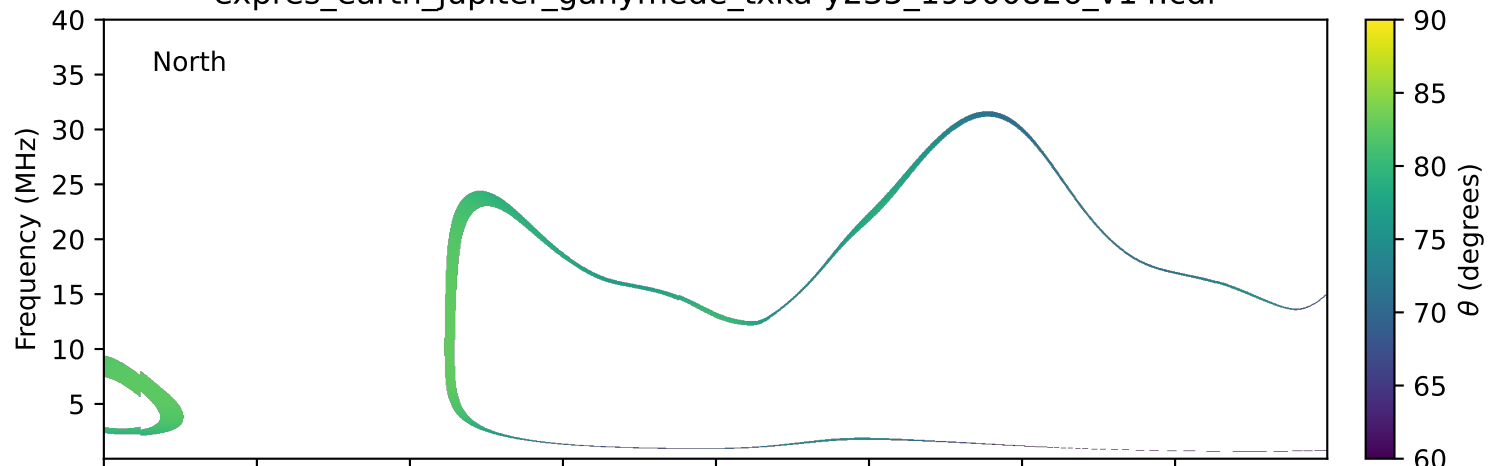
expres_earth_jupiter_ganymede_txka-y235_19900826_v14.cdf
