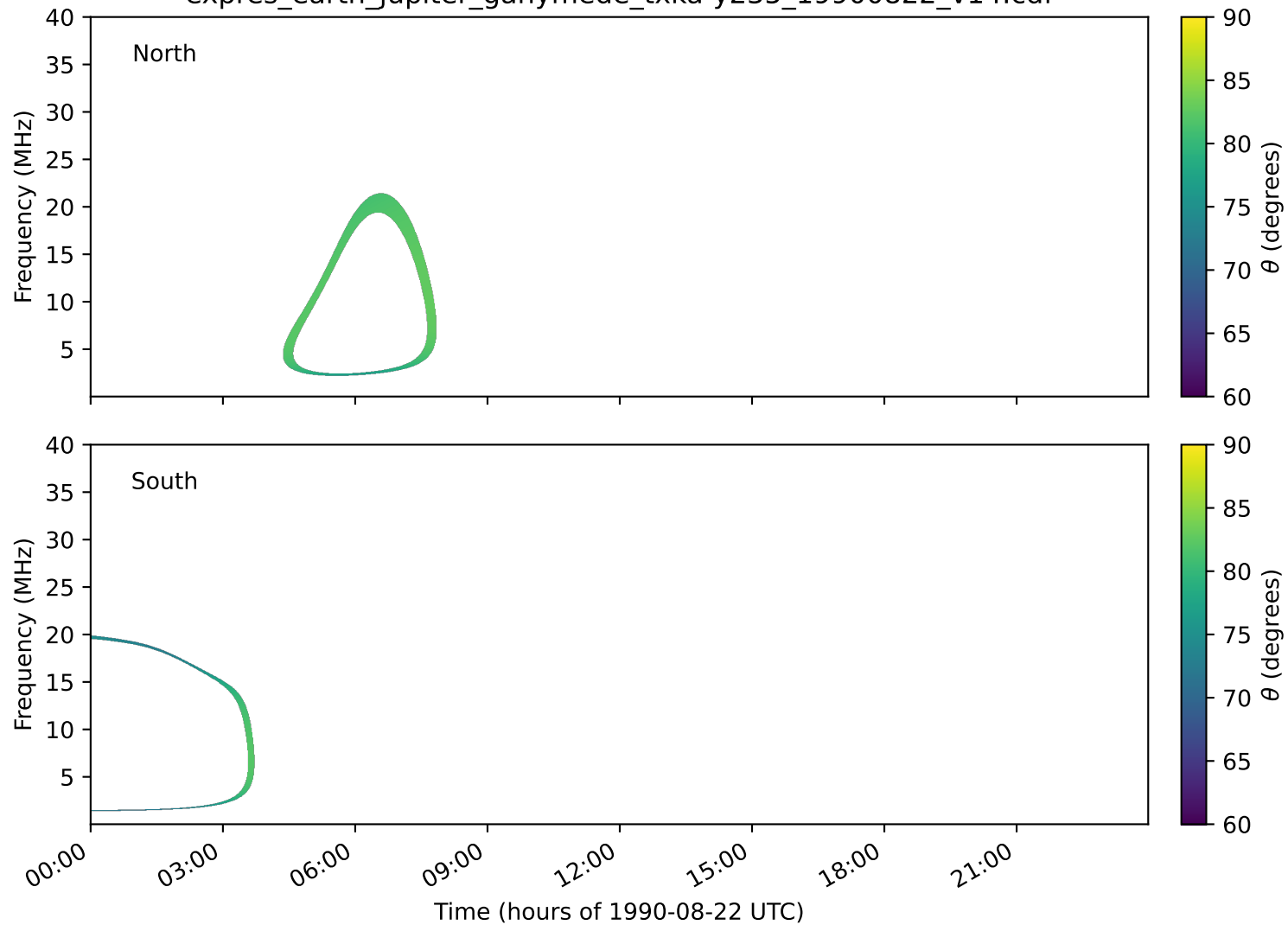
expres_earth_jupiter_ganymede_txka-y235_19900822_v14.cdf
