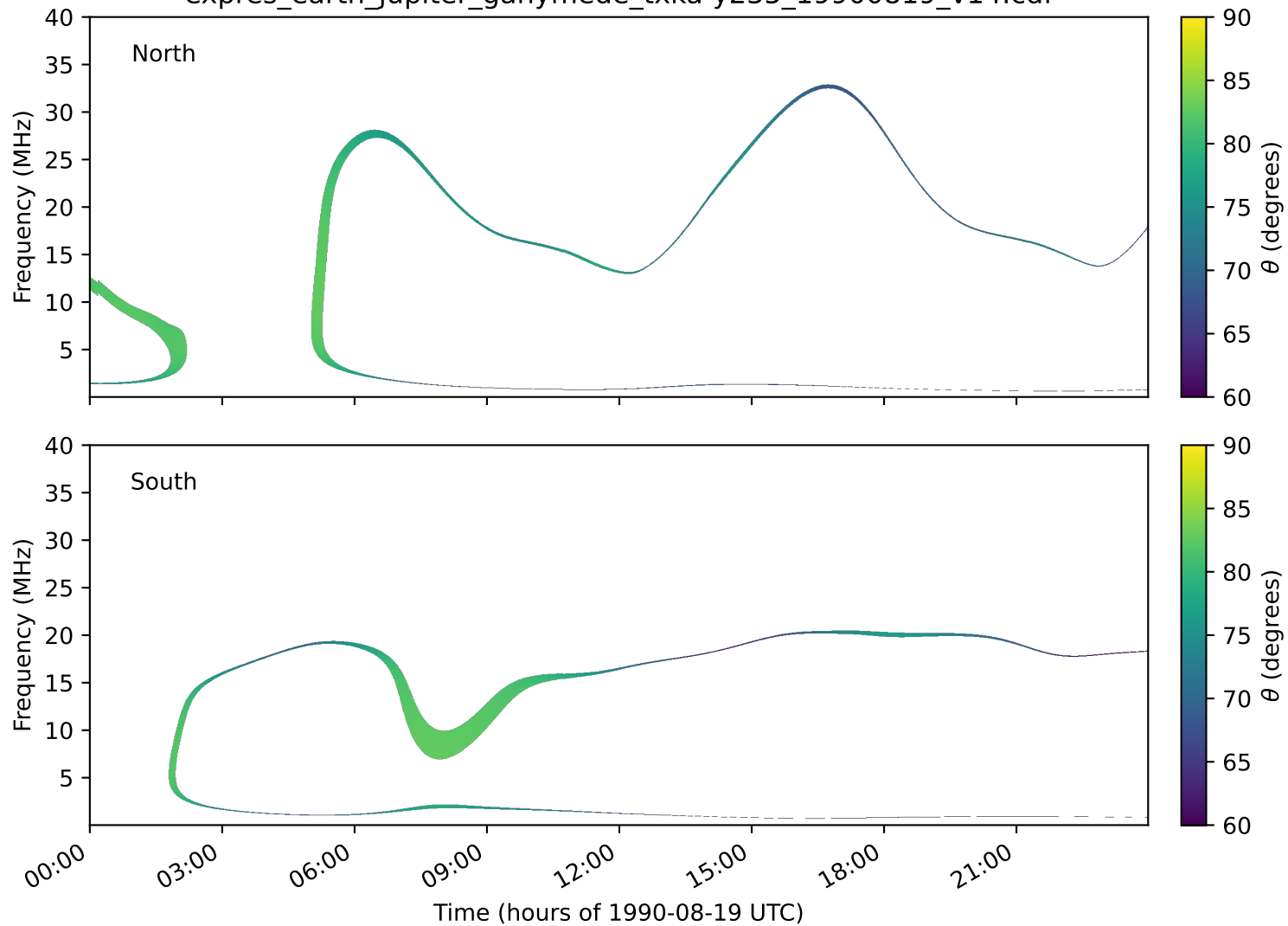
expres_earth_jupiter_ganymede_txka-y235_19900819_v14.cdf
