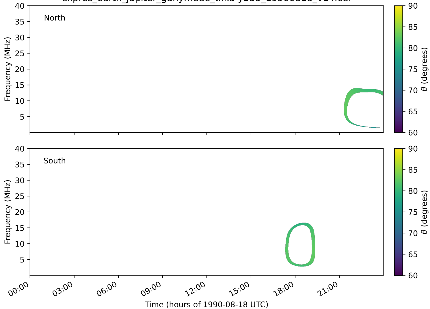
expres_earth_jupiter_ganymede_txka-y235_19900818_v14.cdf
