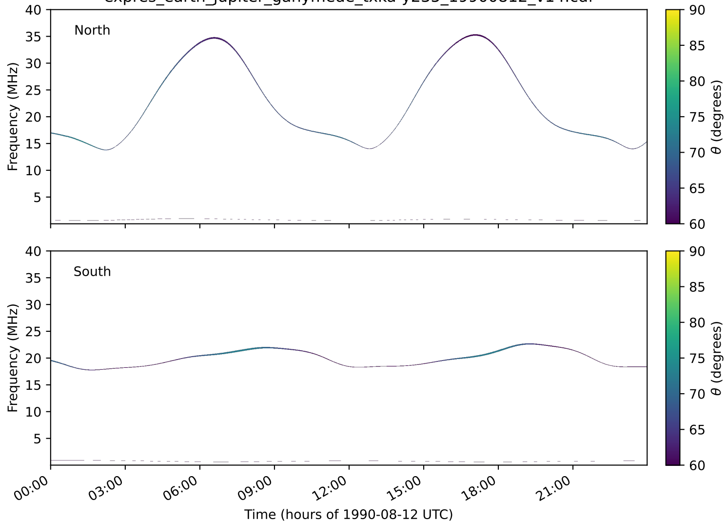
expres_earth_jupiter_ganymede_txka-y235_19900812_v14.cdf
