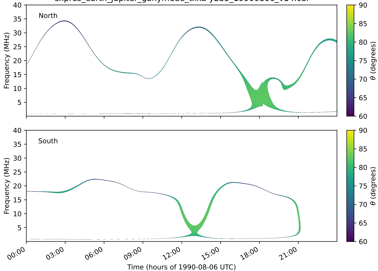
expres_earth_jupiter_ganymede_txka-y235_19900806_v14.cdf
