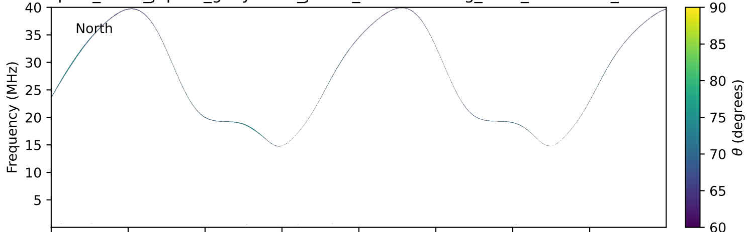
expres_earth_jupiter_ganymede_jrm33_lossc-wid1deg_3kev_19900820_v11.cdf
