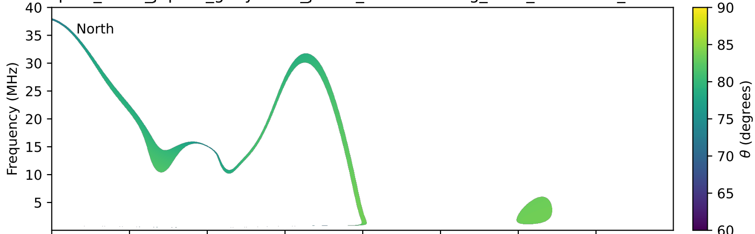
expres_earth_jupiter_ganymede_jrm09_lossc-wid1deg_3kev_19900814_v11.cdf
