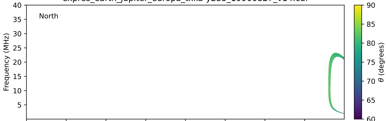
expres_earth_jupiter_europa_txka-y235_19900827_v14.cdf
