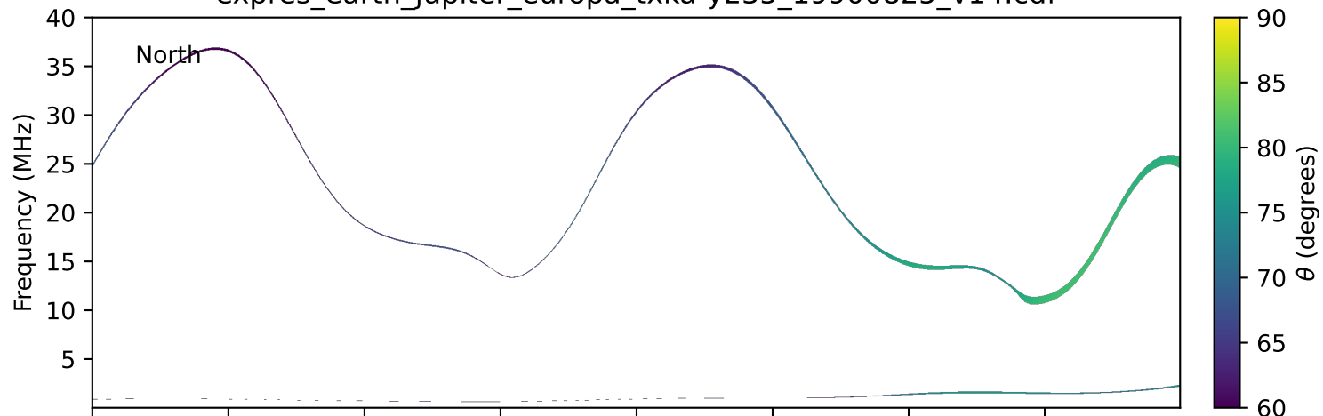
expres_earth_jupiter_europa_txka-y235_19900825_v14.cdf
