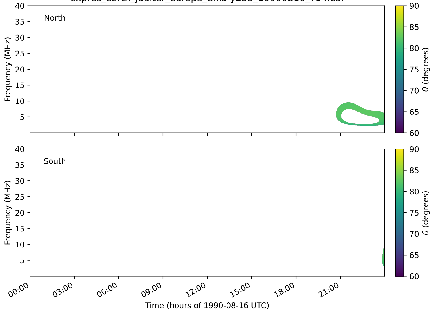
expres_earth_jupiter_europa_txka-y235_19900816_v14.cdf
