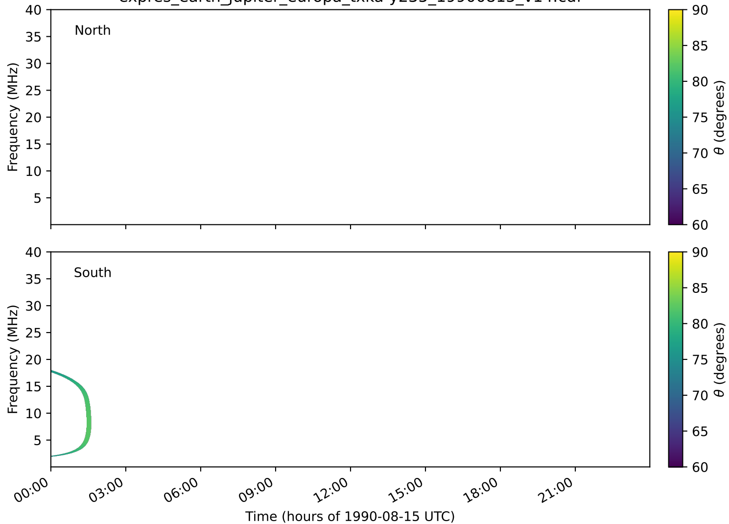
expres_earth_jupiter_europa_txka-y235_19900815_v14.cdf
