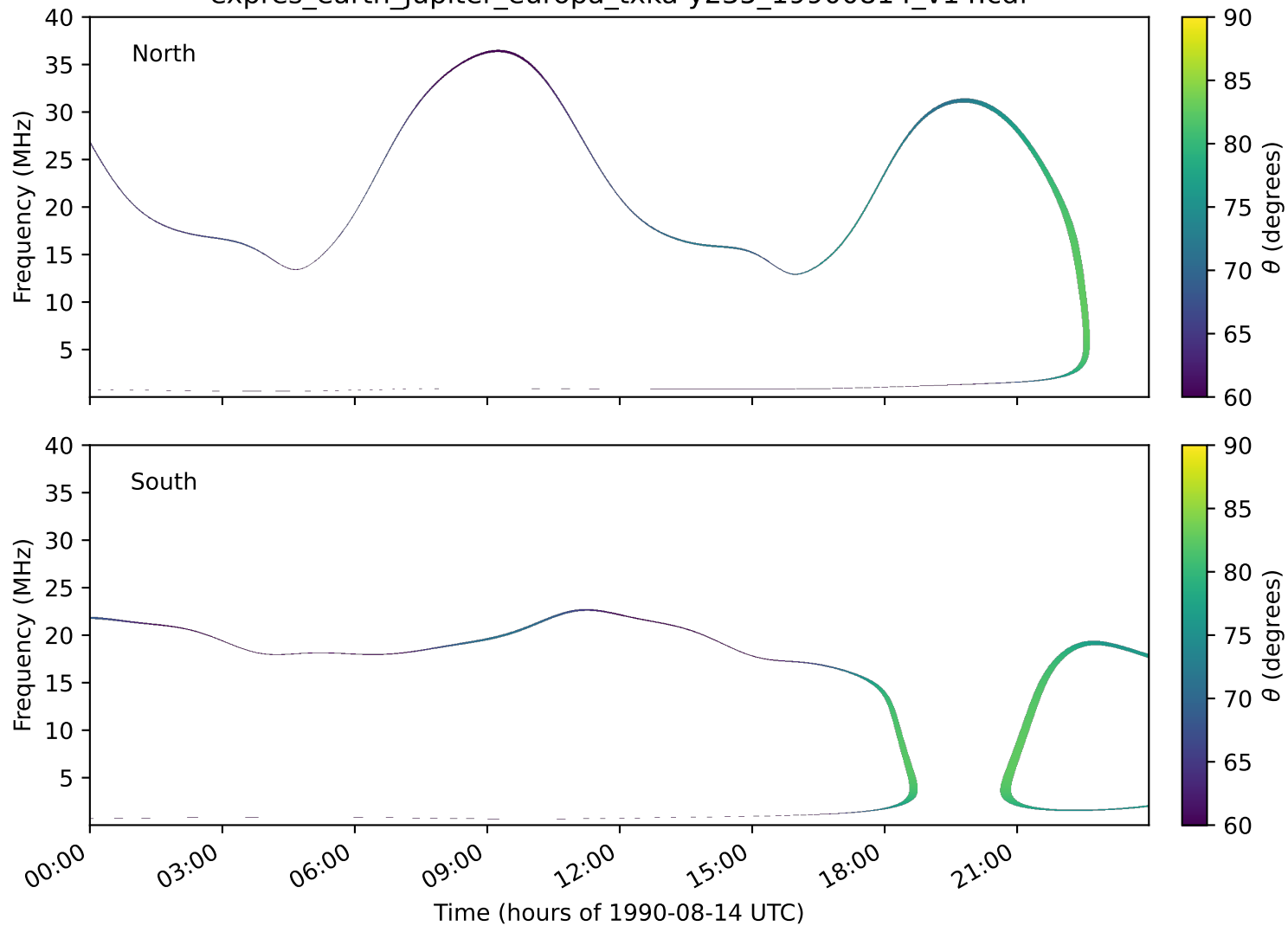
expres_earth_jupiter_europa_txka-y235_19900814_v14.cdf
