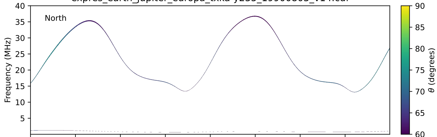
expres_earth_jupiter_europa_txka-y235_19900803_v14.cdf
