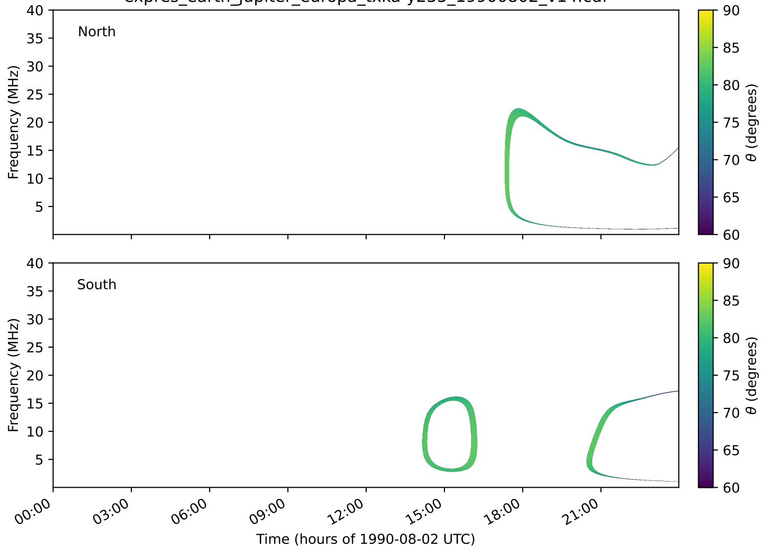
expres_earth_jupiter_europa_txka-y235_19900802_v14.cdf
