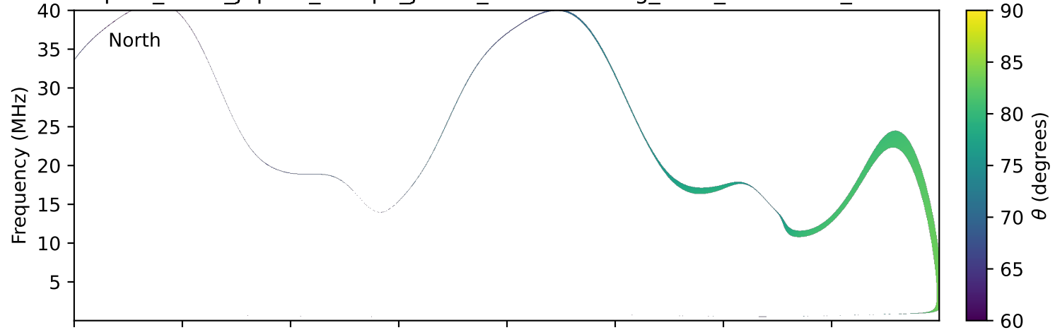
expres_earth_jupiter_europa_jrm33_lossc-wid1deg_3kev_19900818_v11.cdf
