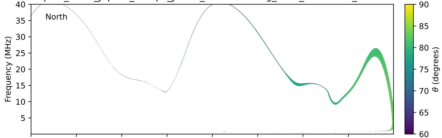
expres_earth_jupiter_europa_jrm09_lossc-wid1deg_3kev_19900818_v11.cdf
