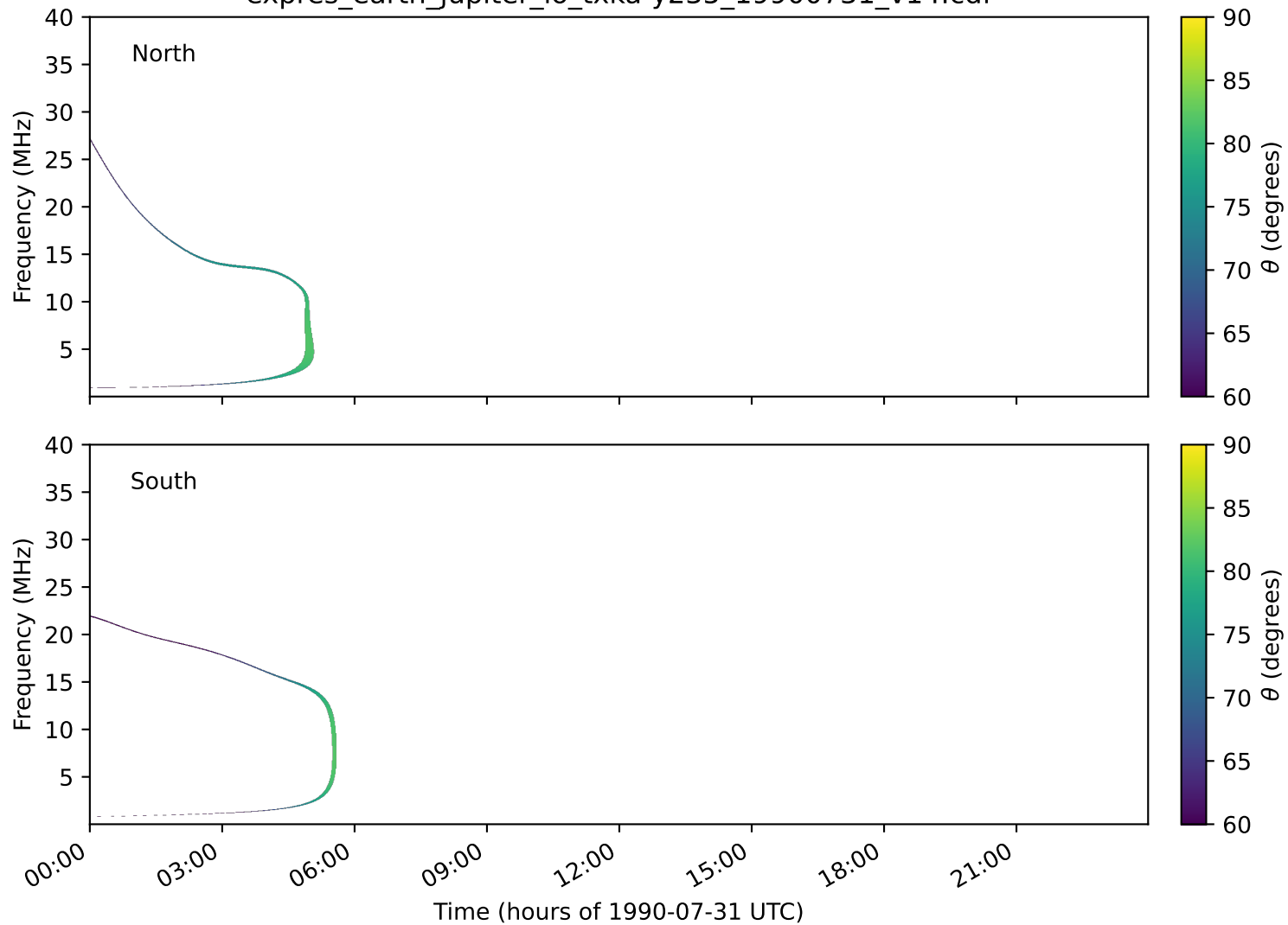
expres_earth_jupiter_io_txka-y235_19900731_v14.cdf
